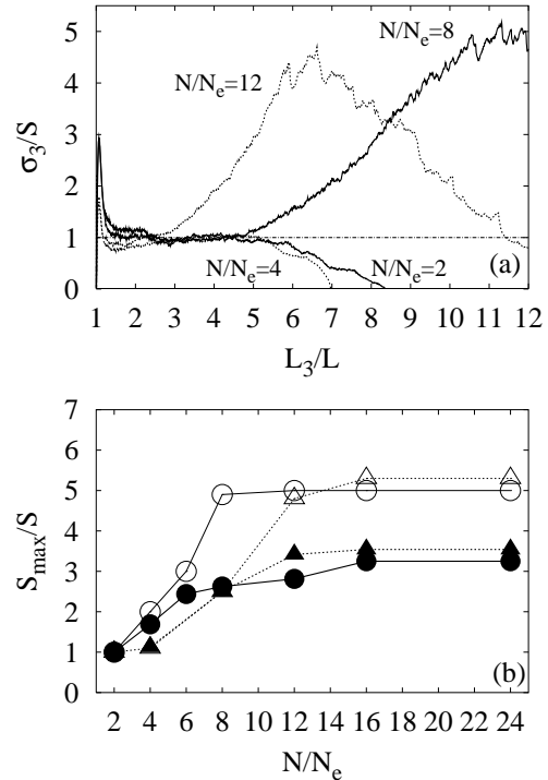
FIG. 2. (a) Normalized stress \sigma_3/S during craze growth at T = 0.3 u_0/k_B for flexible (solid lines) and semiflexible (dotted lines) chains of the indicated length in systems composed of 32768 beads. Here we take N_e = 32 for the semiflexible and N_e = 64 for the flexible chains. The value of S_{\max}/S is obtained from the maximum height of the curves. Panel (b) summarizes S_{\max}/S for the flexible (o) as well as semiflexible ( \Delta ) chains at T = 0.3 u_0/k_B (open symbols) and T = 0.1 u_0/k_B (filled symbols) as a function of chain length.
